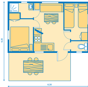
EVASION MOBILE HOME / 4 persons - 24 m 2 + terrace 10 m 2
